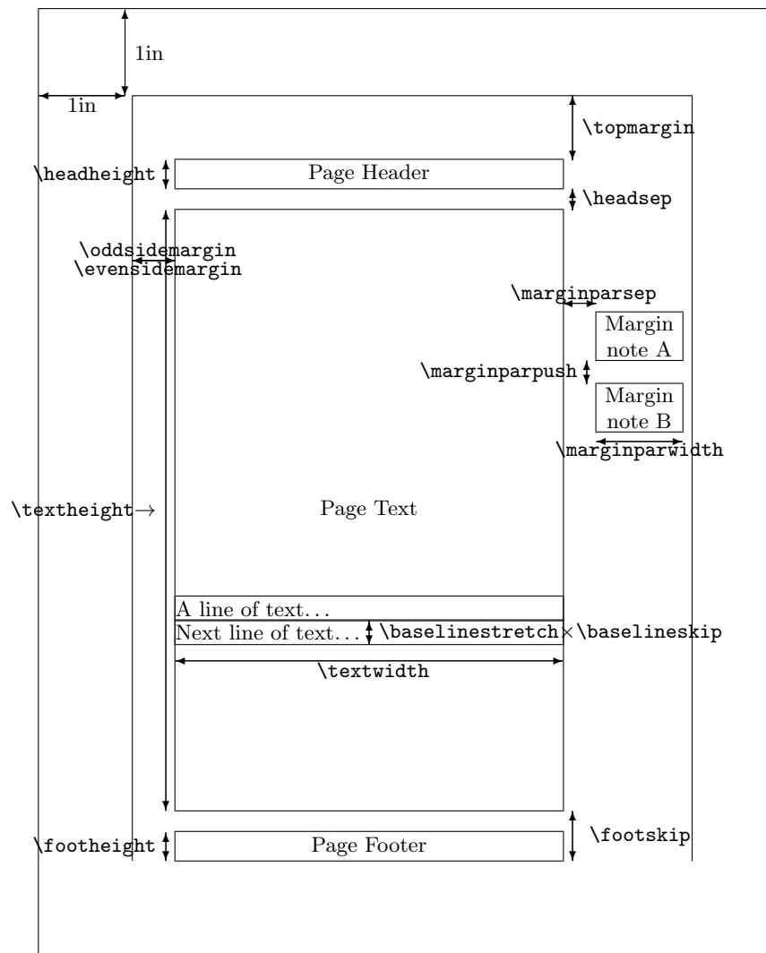
Figure 1: \text{\LaTeX} single-column page layout. The actual proportions correspond to parameter values in the 11pt BOOK document style. Note that standard-conforming DVI drivers are required to place the \text{\TeX} upper-left page corner one inch over and down from the corner of the physical output page. This figure is scaled to 50% of actual page size. It was produced on October 3, 2018 at 8:01.
