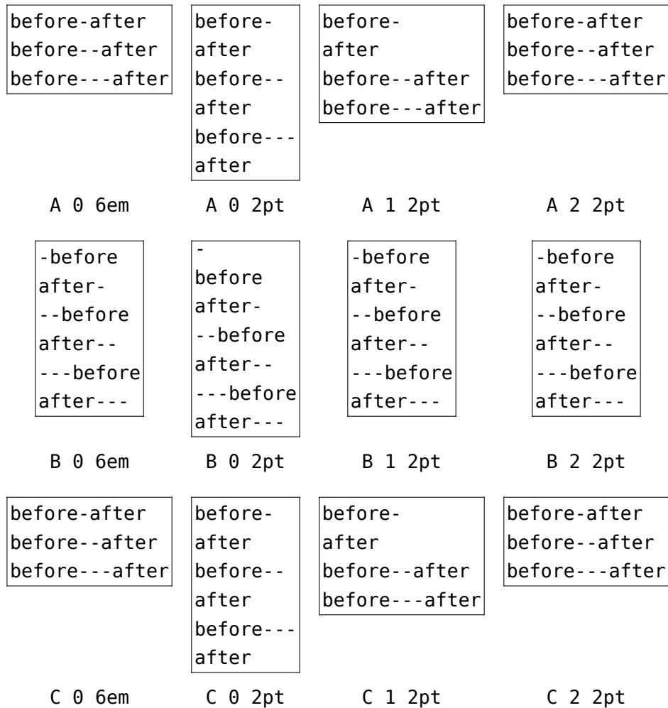
Figure 5.6 The automatic modes 0 (default), 1 and 2, with a \hsize of 6em and 2pt (which triggers a linebreak).
