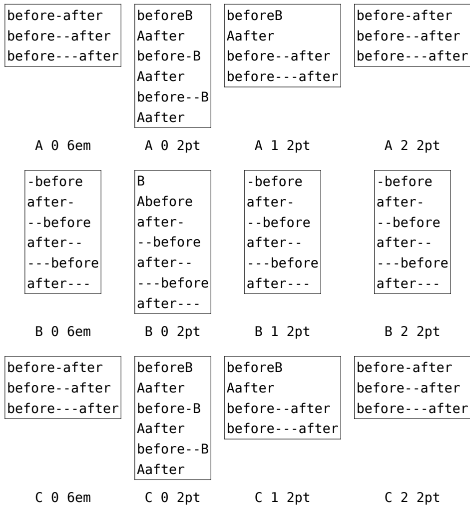
Figure 5.7 The automatic modes 0 (default), 1 and 2, with \preexhyphenchar and \postexhyphenchar set to characters A and B.
